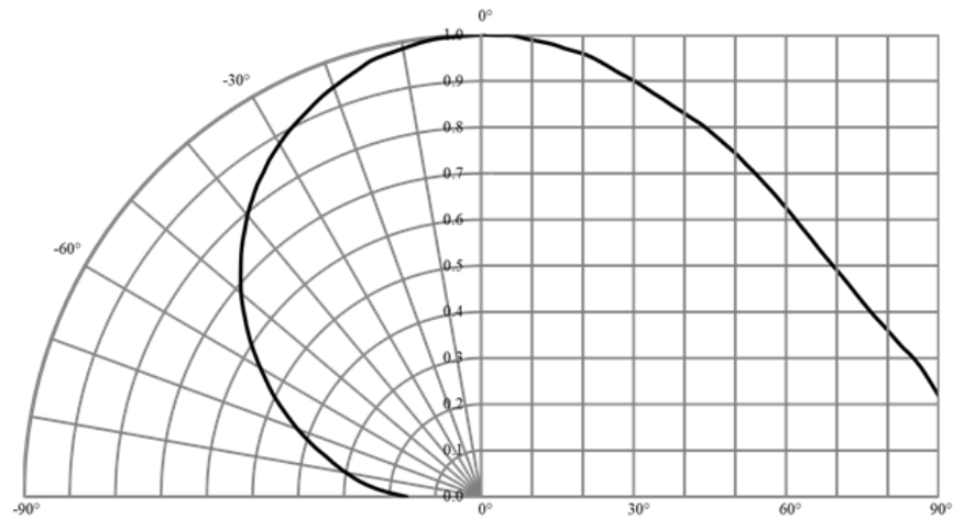
Fig 3. Radiation Characteristics
