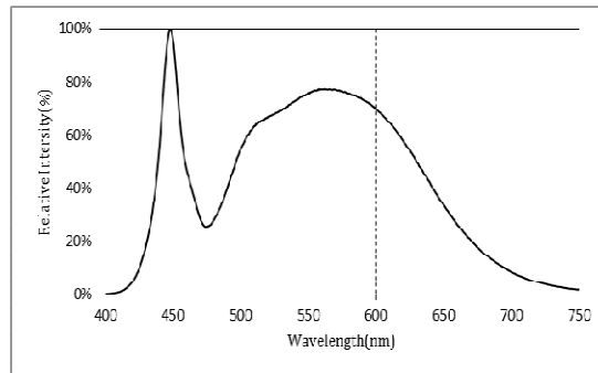
Fig 1. Relative Spectrum of Emission
