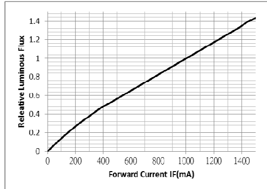
Fig 4. Relative Luminous Flux
