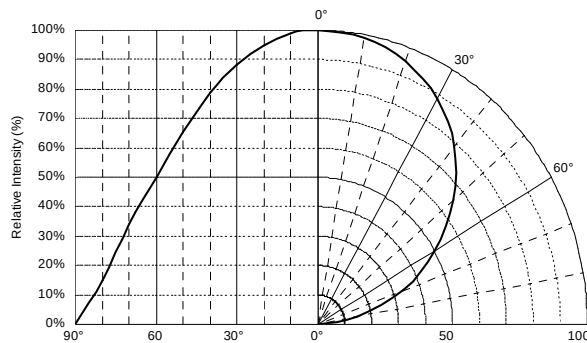
Fig 2. Radiation Characteristics
