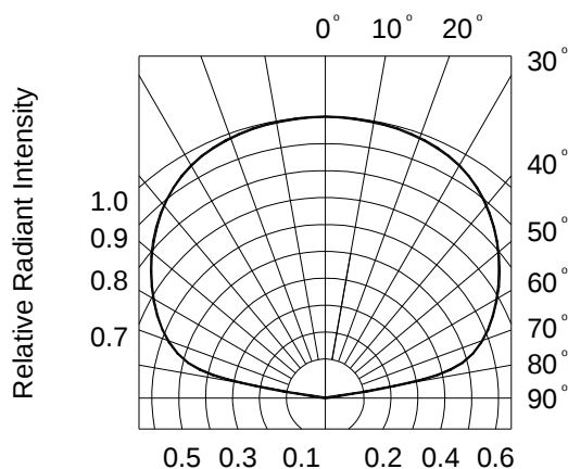
FIG.4 RADIATION DIAGRAM
