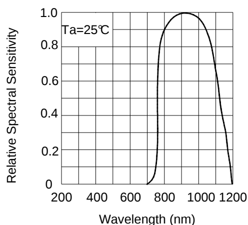
FIG.2 SPECTRAL SENSITIVITY
