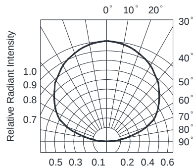
FIG.6 SENSITIVITY DIAGRAM
