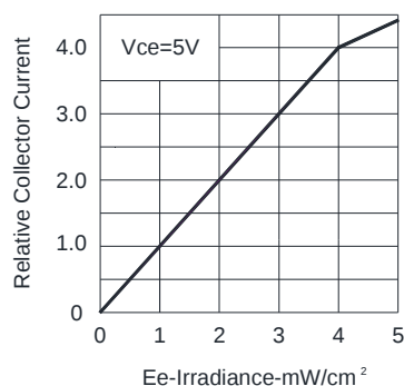
FIG.3 RELATIVE COLLECTOR CURRENT VS IRRADIANCE
