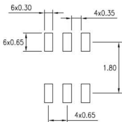
Recommended Land Pattern for LTR-X116A
