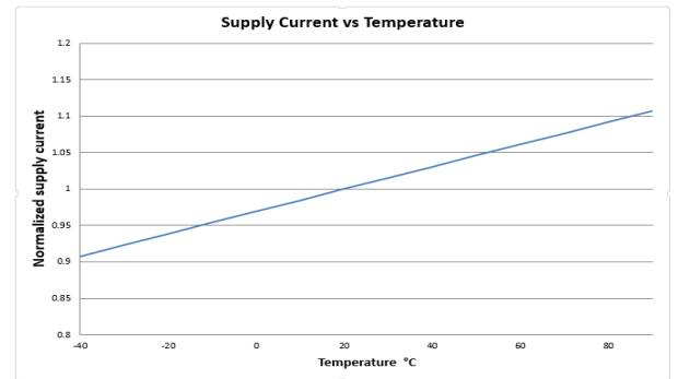
Figure 4.4 Supply Current vs Temperature
