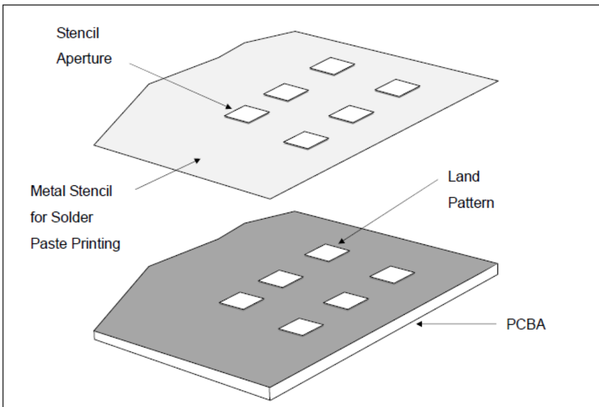
Recommended Land Pattern for LTR-X116A
