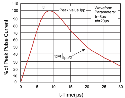
Figure 2. Pulse Waveforms
