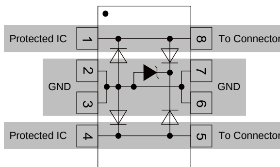
Protection --- Line to GND (Common Mode)
