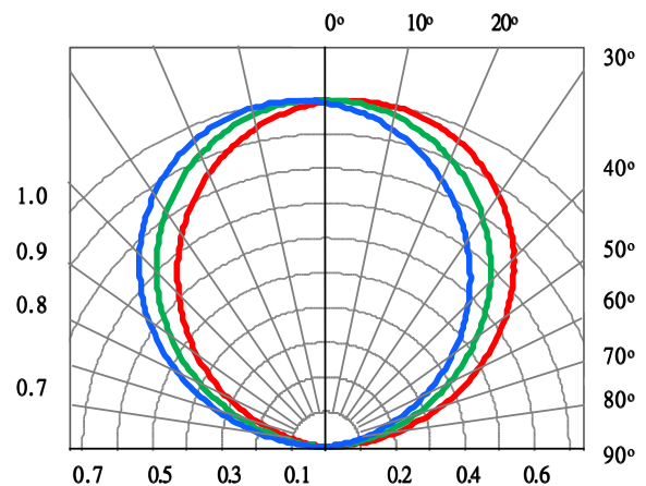
Fig. 3 Spatial Distribution
