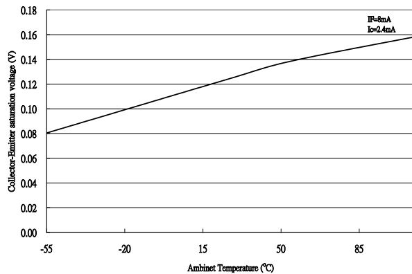
Figure 13. Collector-Emitter Saturation Voltage vs. Ambient Temperature
