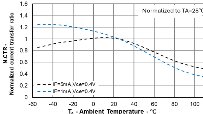
Figure 12. Normalized Current Transfer Ratio vs. Ambient Temperature (Vce=0.4V)
