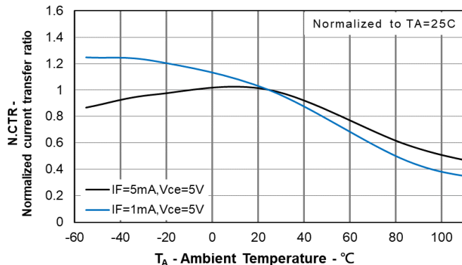
Figure 11. Normalized Current Transfer Ratio vs. Ambient Temperature (Vce=5V)
