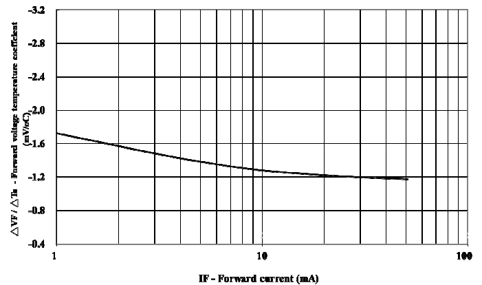
Figure 4. Forward Voltage Temperature Coefficient vs. Forward Current
