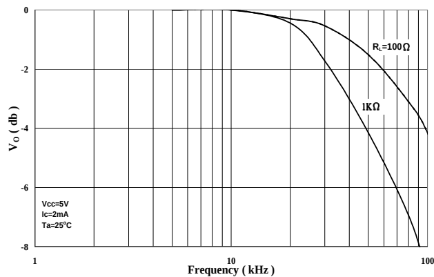
Figure 17. Frequency Response
