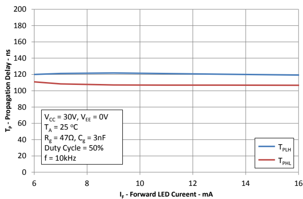
Figure 9: Propagation Delays vs. I_F
