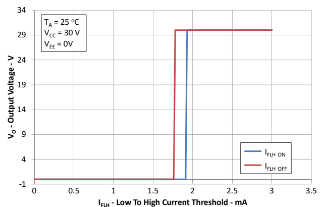
Figure 6: IFLH hysteresis
