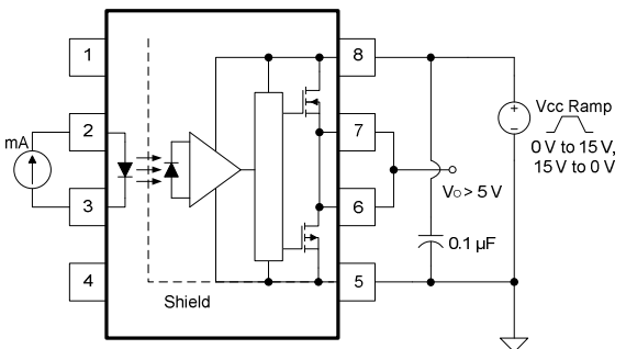
Figure 19 : UVLO Test Circuit
