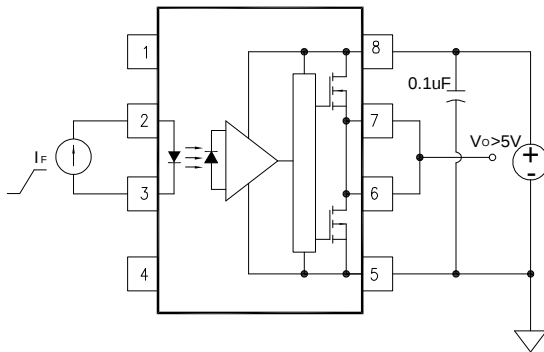
Figure 18 : I_{FLH} Test Circuit
