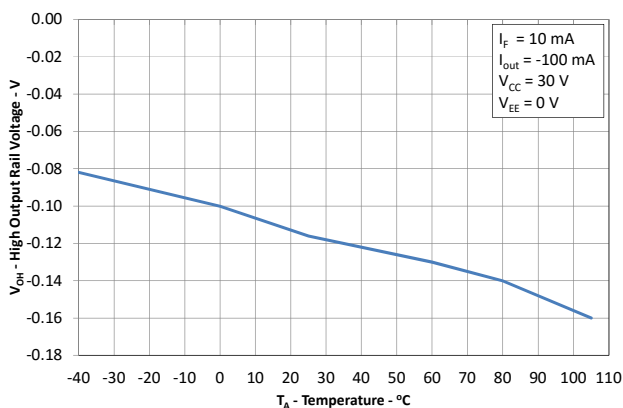
Figure 2: V_{OH} vs. Temperature
