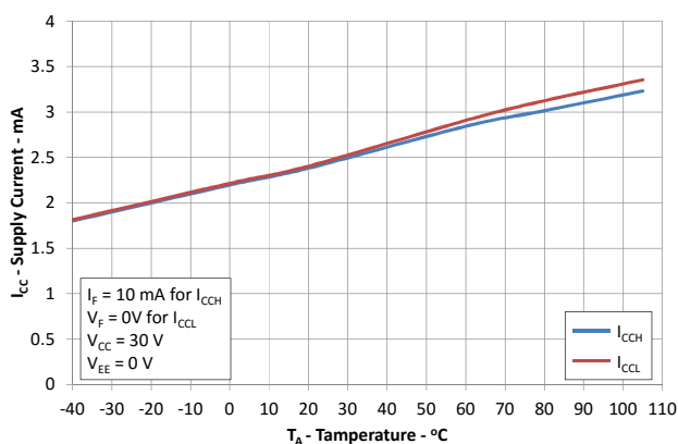
Figure 4: I_{CC} vs. Temperature
