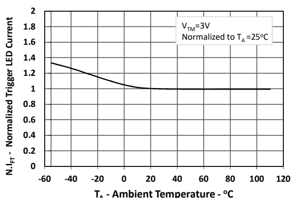
Fig.3 Normalized Trigger Current vs Ambient Temperature
