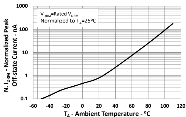
Fig.9 Leakage in Inhibited State vs Ambient Temperature
