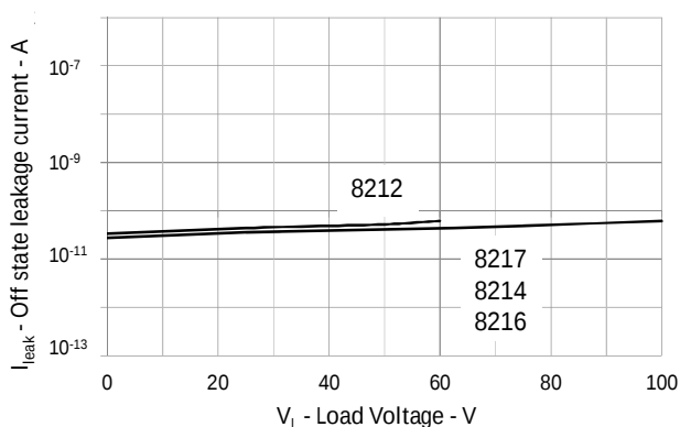
Fig. 9. Off State Leakage Current vs. Load Voltage
