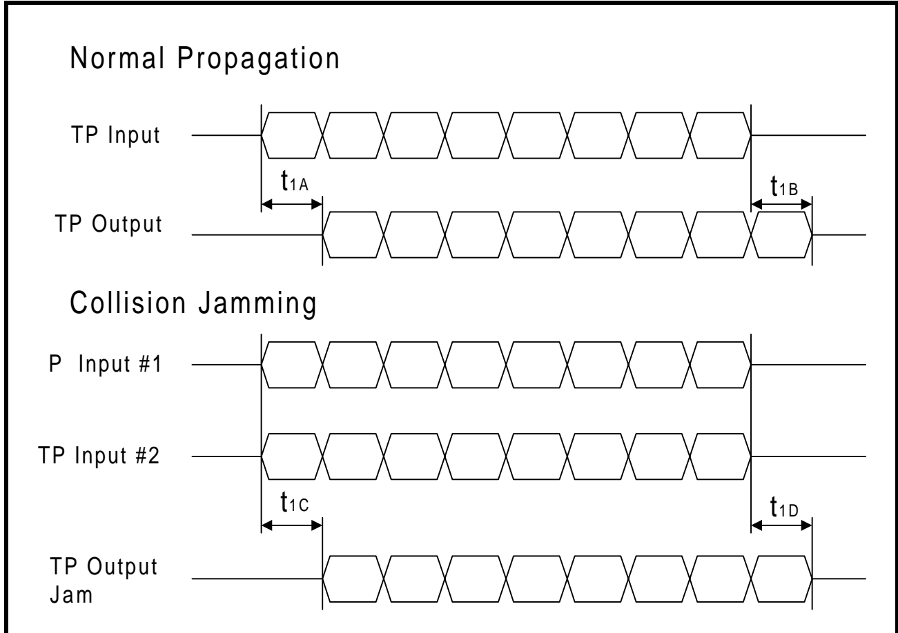
Figure 17: 100 Mbps TP Port-to-Port Delay Timing
