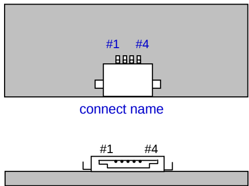
Fig. Connector diagram
