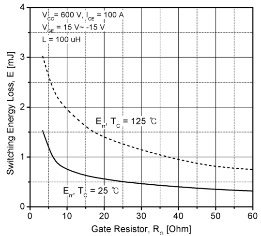
Fig 14. Typical Diode Switching Loss
