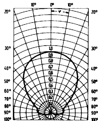
2I. Radiation characteristic I_{REL} = f(\varphi)
