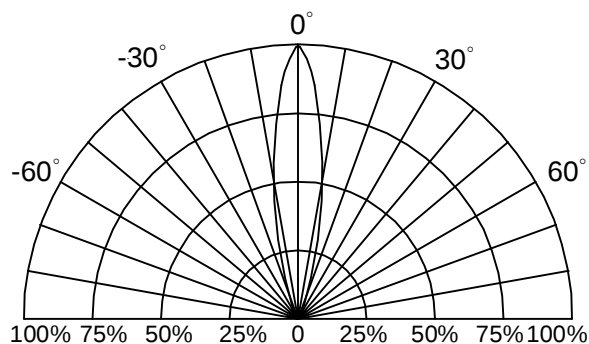
Fig.6 Directivity Radiation
