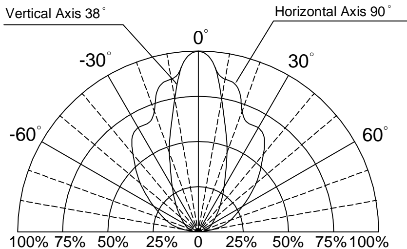
Radiation Angle(0.5):H 90 Degree/V 38 Degree
