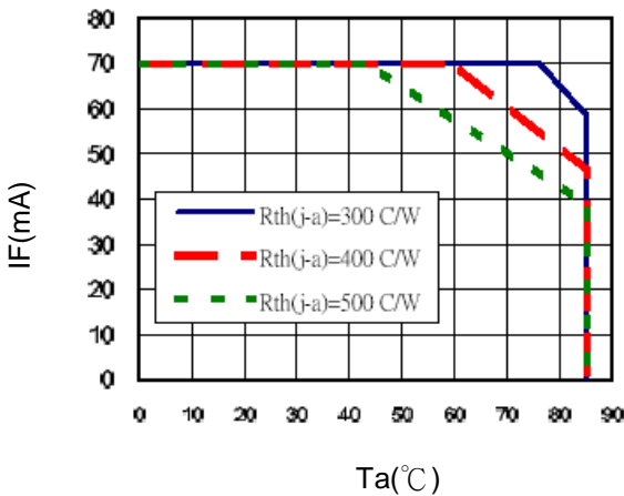
Fig.3 Derating curve based on Tj(max)125 °C
