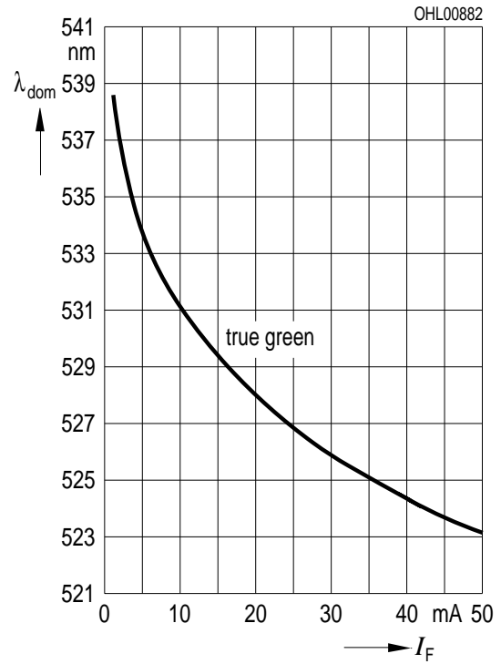
Dominante Wellenlänge \lambda_{\text{dom}} = f(I_F) Dominant Wavelength LT, T_A = 25^\circ\text{C}
