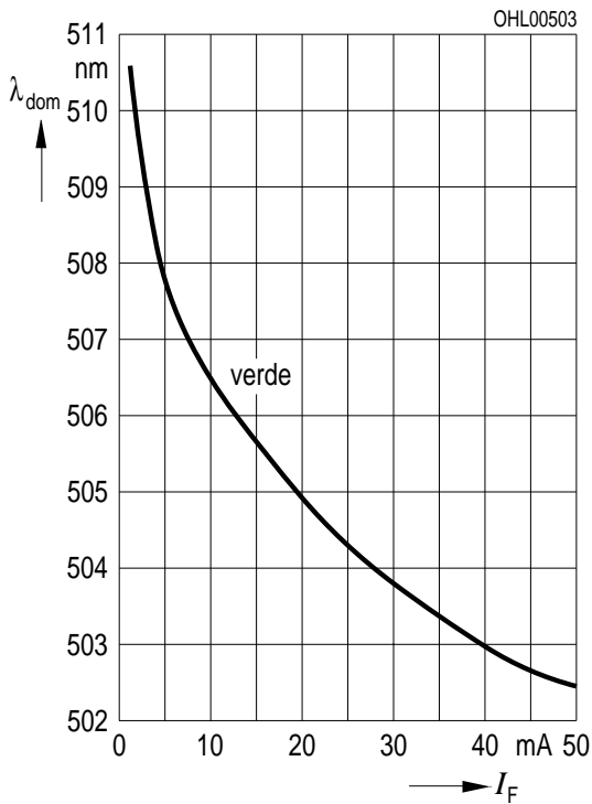
Dominante Wellenlänge \lambda_{\text{dom}} = f(I_F) Dominant Wavelength LV, T_A = 25^\circ\text{C}
