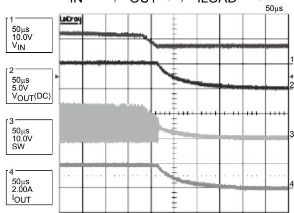
Shutdown Waveform VIN=12V, VOUT=5V, RLOAD=2.67Ω
