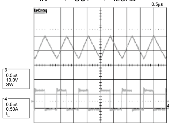
Operating Waveform VIN=12V, VOUT=5V, RLOAD=2.67Ω
