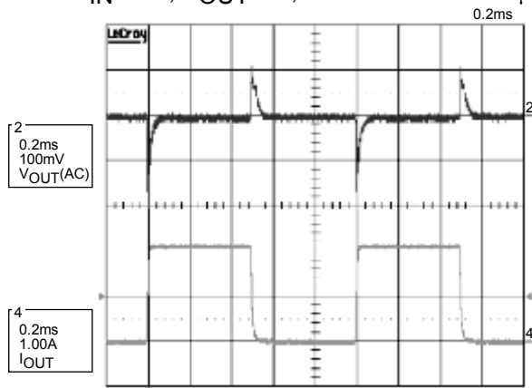
Load Step Waveform VIN=12V, VOUT=5V, ILOAD=0 ⇔ 2.1A/10μs
