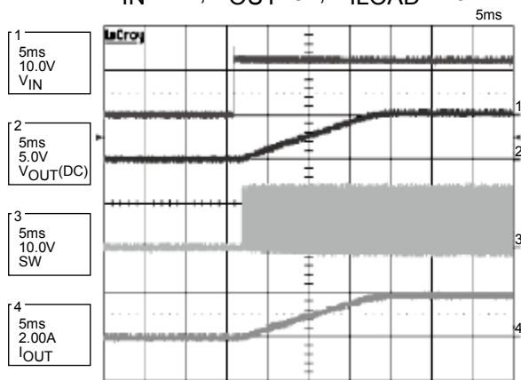
Start up Waveform VIN=12V, VOUT=5V, RLOAD=2.67Ω
