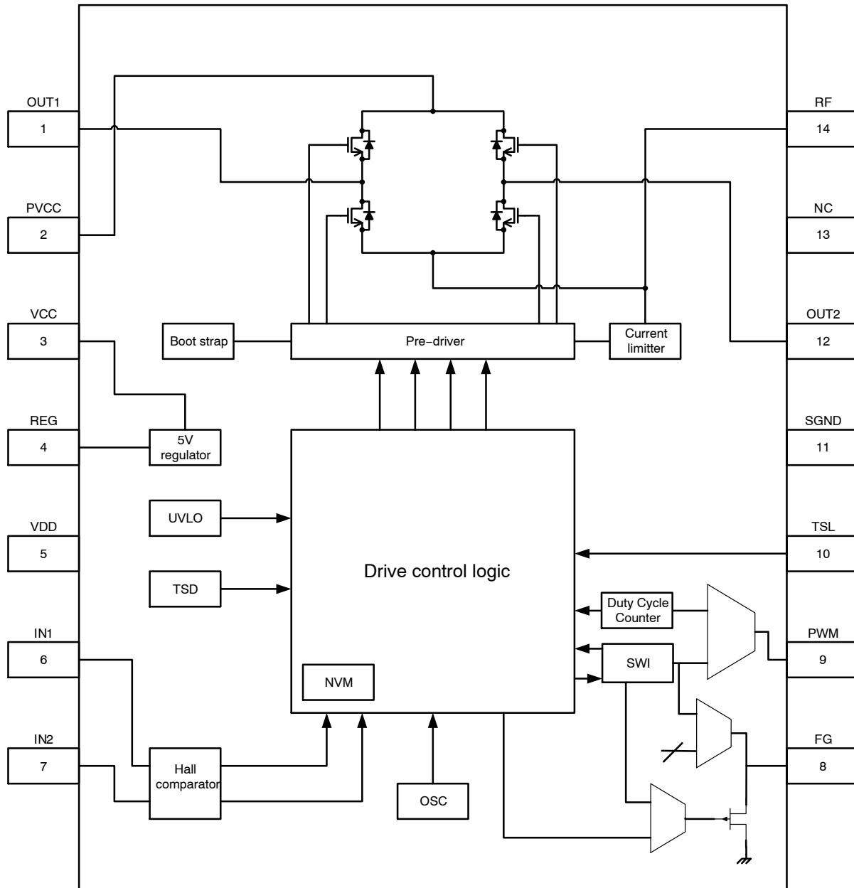
Figure 2. Block Diagram
