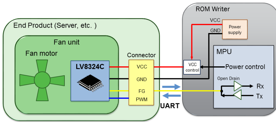
Figure 23. Connection Image of One-wire Mode UART
