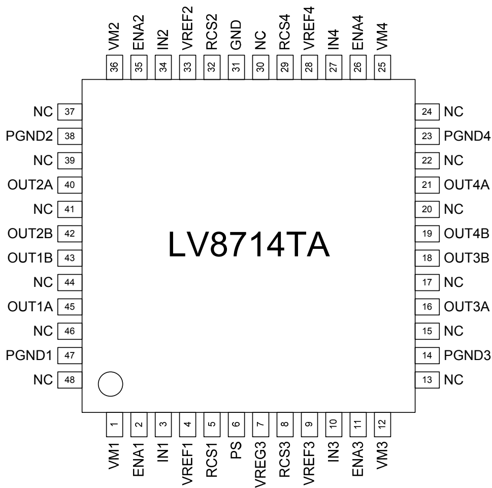
Figure 5. Pin Assignment
