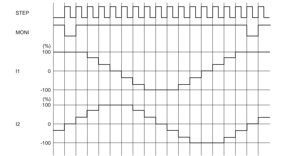
W1-2 phase excitation (CW mode)
