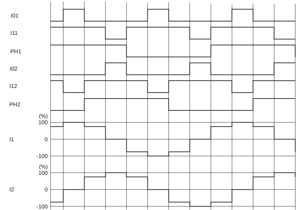
Half step (CW mode)
