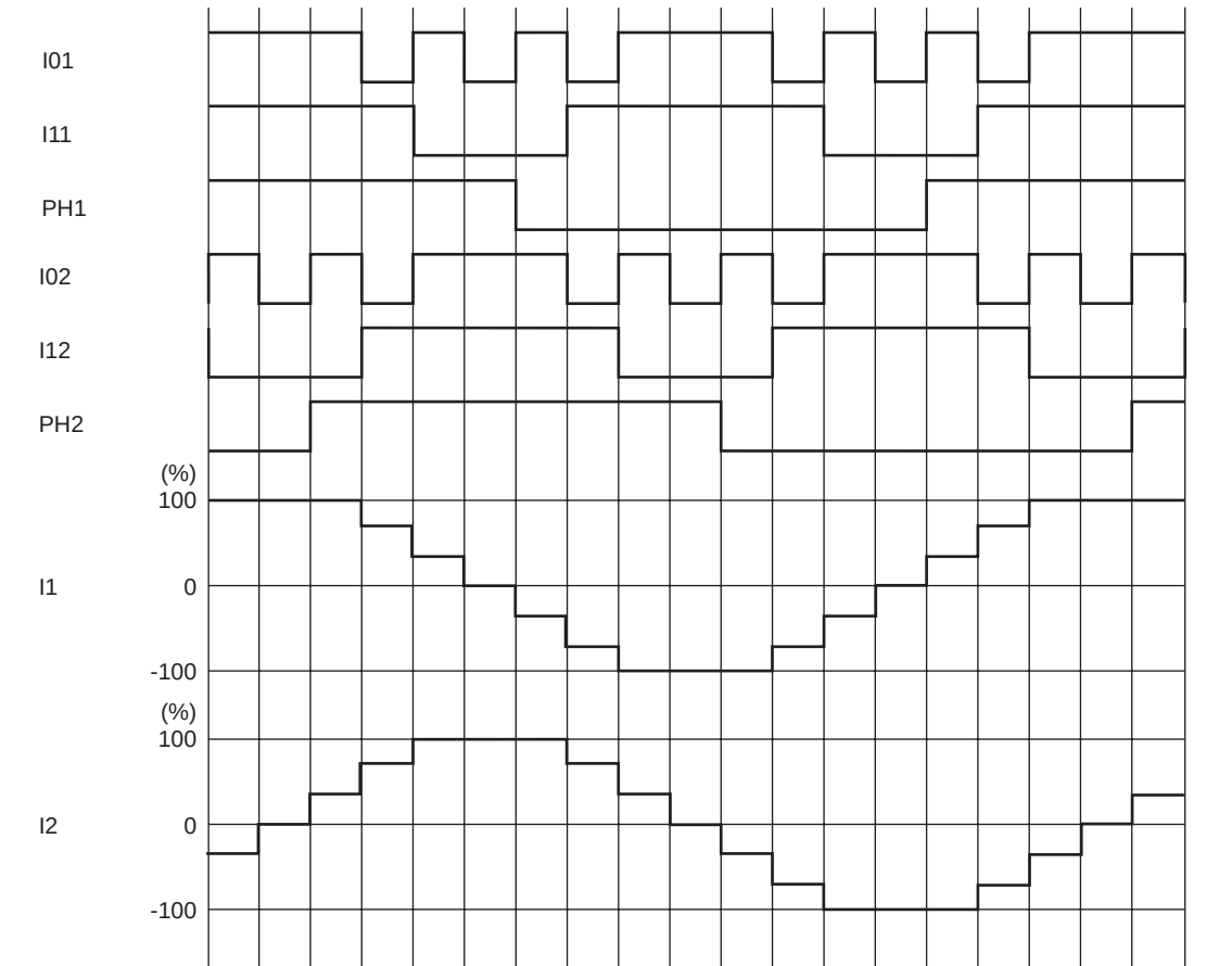
Quarter step (CW mode)
