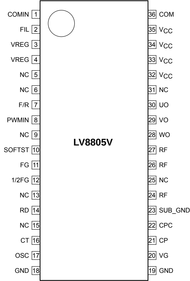
Top view
