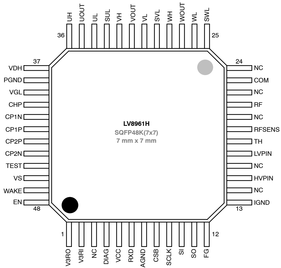
Figure 4. LV8961H Pinout
