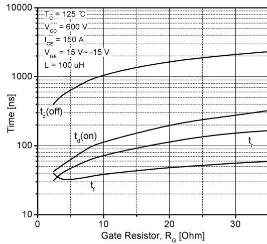
Fig 8. Typical Switching Time vs. Gate Resistor
