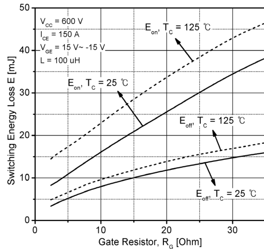
Fig 10. Typical IGBT Switching Loss
