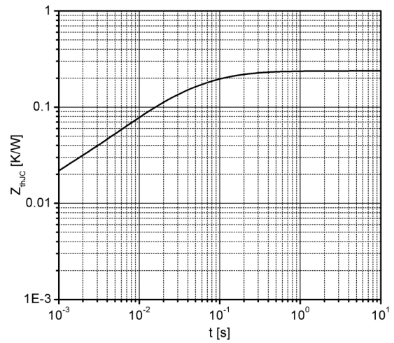
Fig 16. Typical Transient Thermal Impedance
