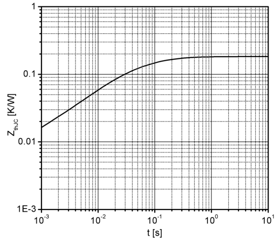
Fig 16. Typical Transient Thermal Impedance
