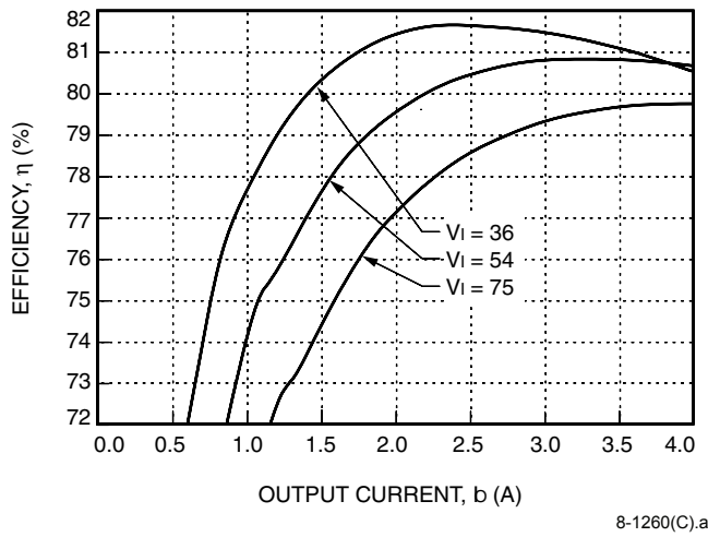
Figure 5. LW020A Typical Converter Efficiency vs. Output Current
