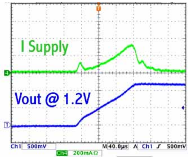
Figure 7– Soft Start Power On, L = 2.7µH, C_{OUT} = 30µF, I_{OUT} = 0mA DC
