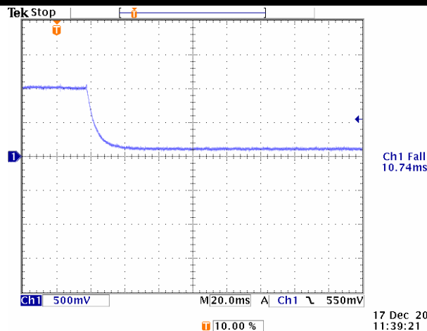
Chart 1 & 2 – Step Response Graphs VDD = 4V, 200 to 20 Lux step 30.3K Load resistance
