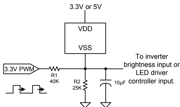
Figure 5 – Semi-Manual Controlled Dimming
