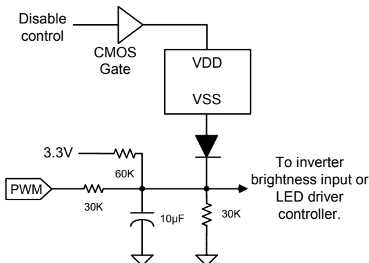
Figure 6 – Fully Manual Controlled Dimming
