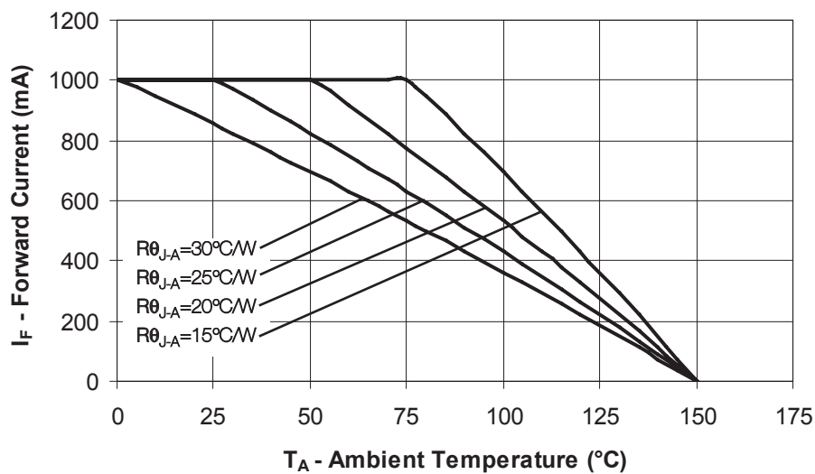
Figure 19: Maximum forward current vs. ambient temperature, based on T JMAX = 150°C.
