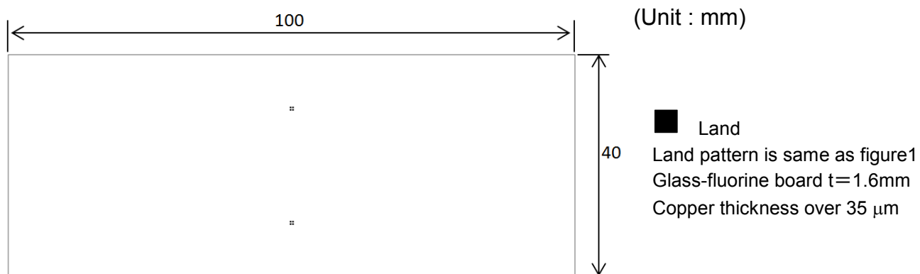
Fig. 2 Testing board
