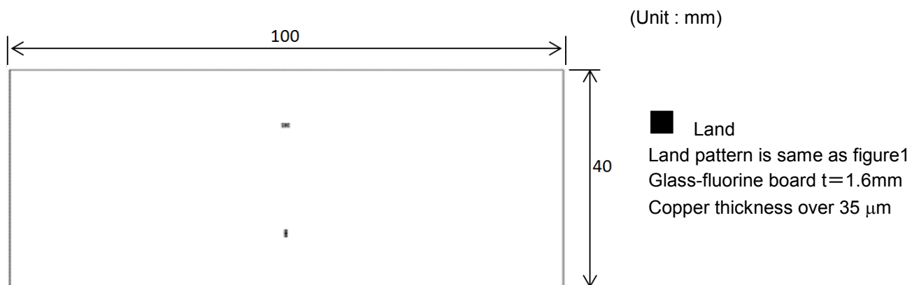
Fig. 2 Testing board
