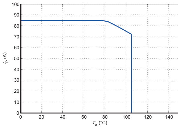
Figure 18: I_p vs T_A for LXSR 25-NPS
