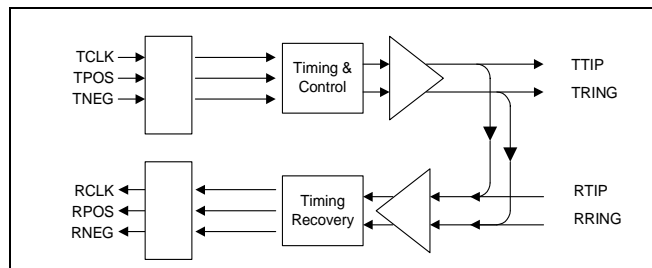
Figure 8. Analog Loopback
