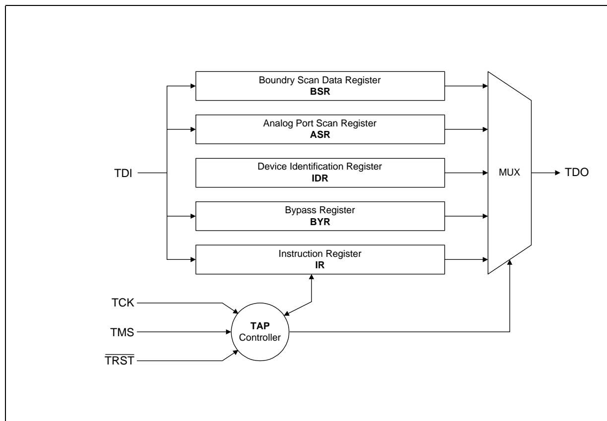
Figure 12. JTAG Architecture
