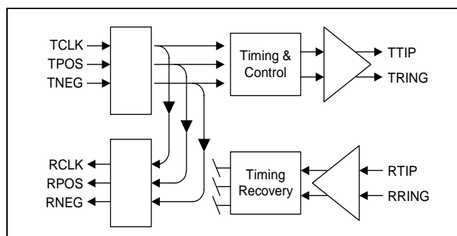
Figure 9. Digital Loopback
