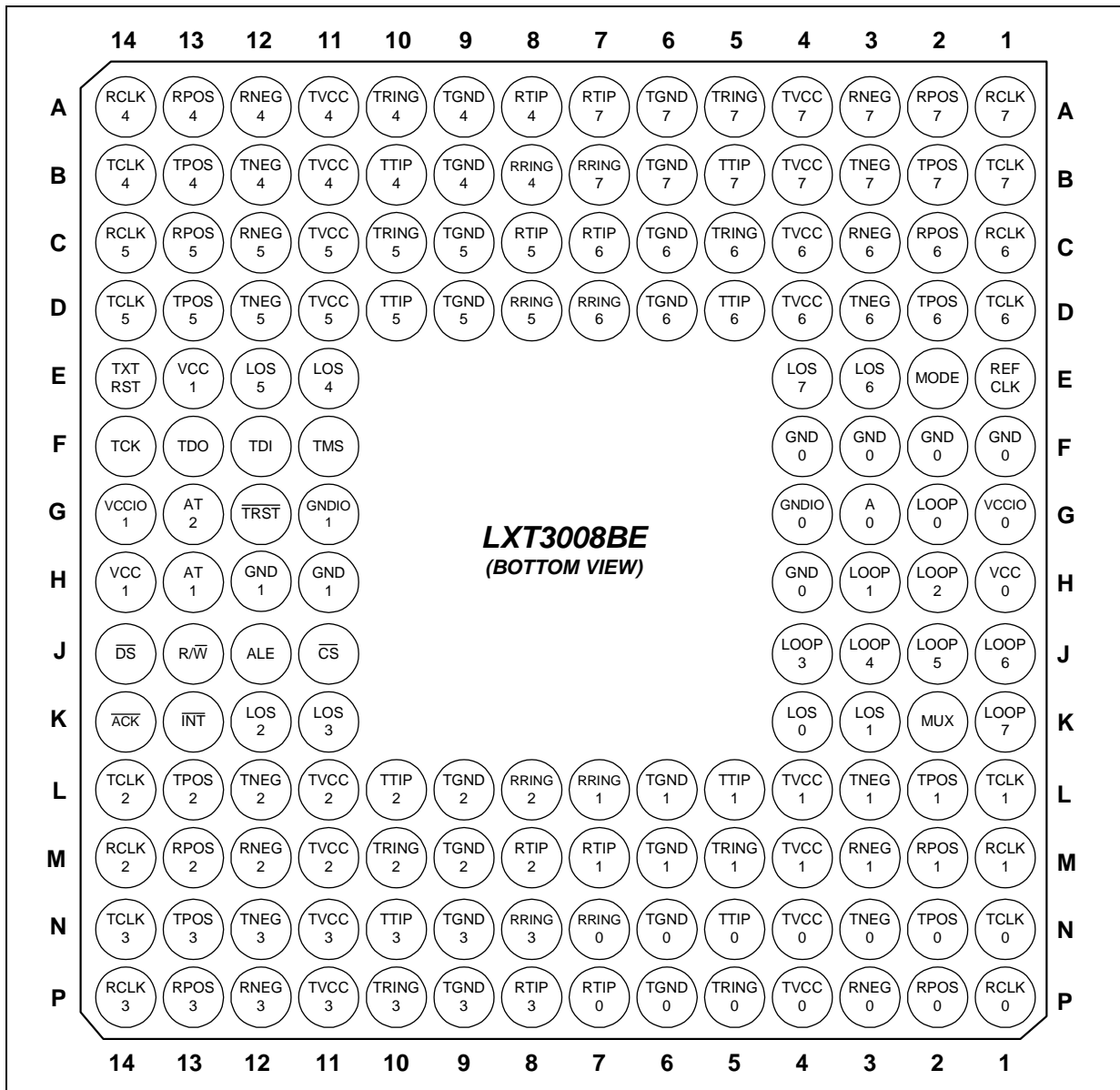
Figure 3. LXT3008 Plastic Ball Grid Array (PBGA) Package Pin Assignments
