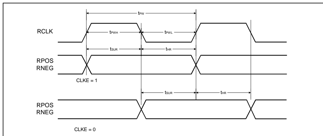
Figure 16. Receive Clock Timing Diagram
