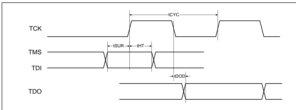
Figure 20. JTAG Timing
