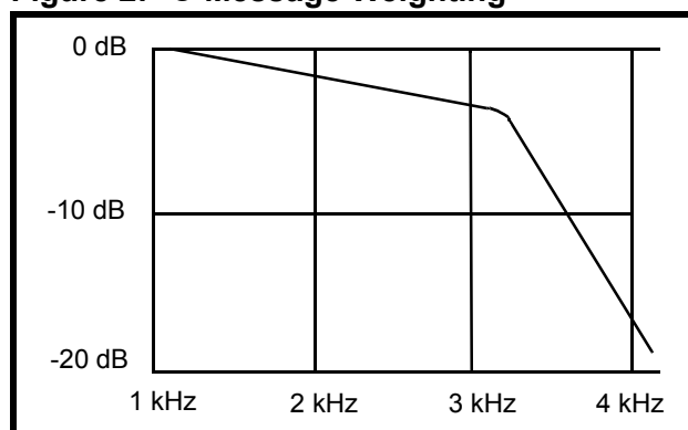
Figure 2: C-Message Weighting
