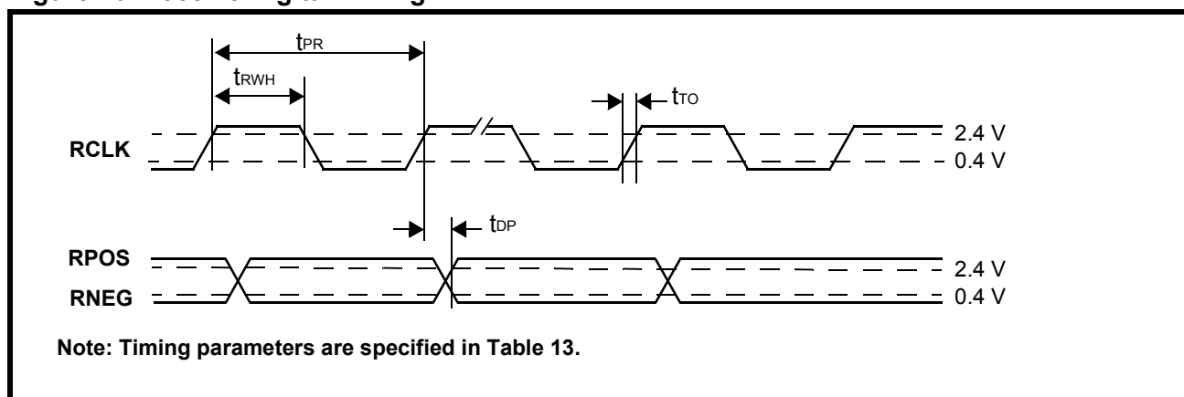
Figure 10: Receive Digital Timing
