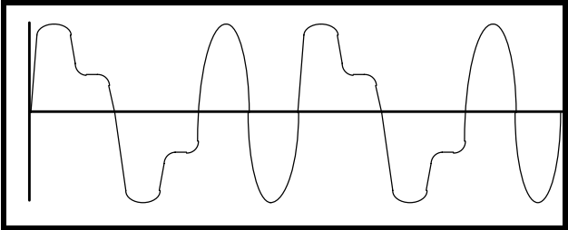
Figure 2: LXT902 TPO Output Waveform
