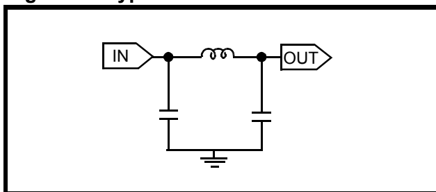
Figure 9: Typical Receive Filter
