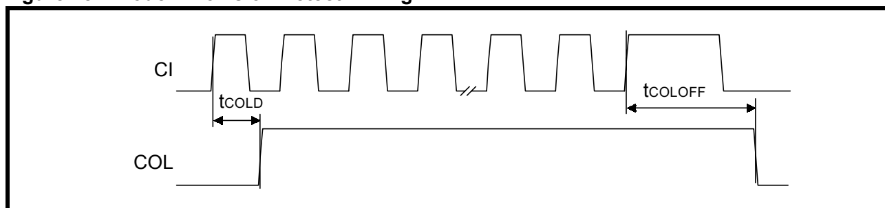
Figure 19: Mode 1 COL/SQE Output Timing/CI Output Timing
