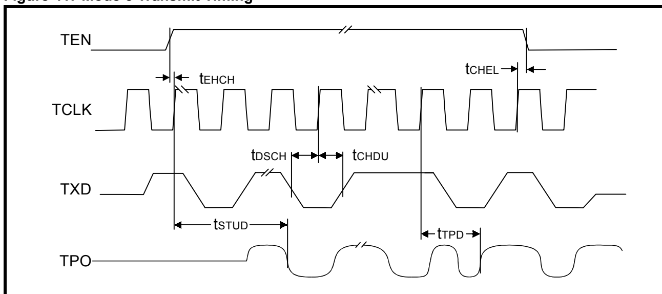
Figure 42: Mode 5 Collision Detect Timing
