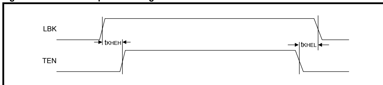
Figure 20: Mode 1 Loopback Timing
