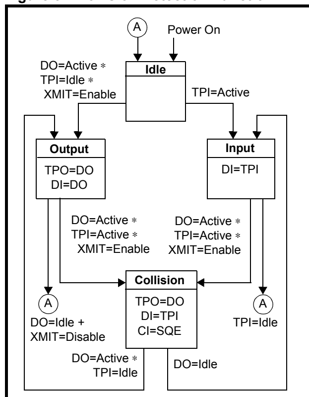
Figure 5: Collision Detection Function
