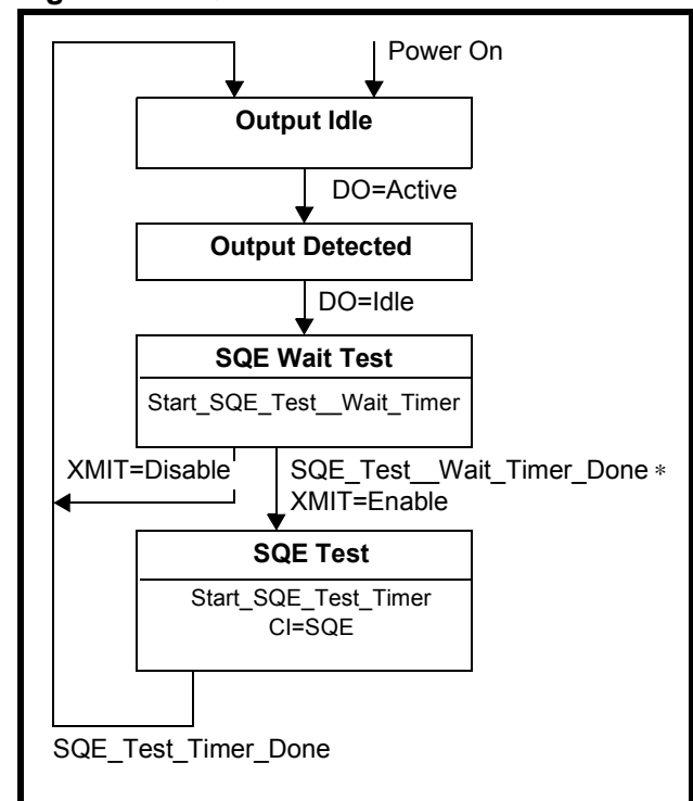
Figure 4: SQE Function
