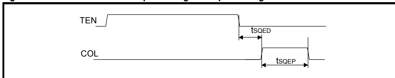
Figure 19: Mode 1 COL/SQE Output Timing/CI Output Timing
