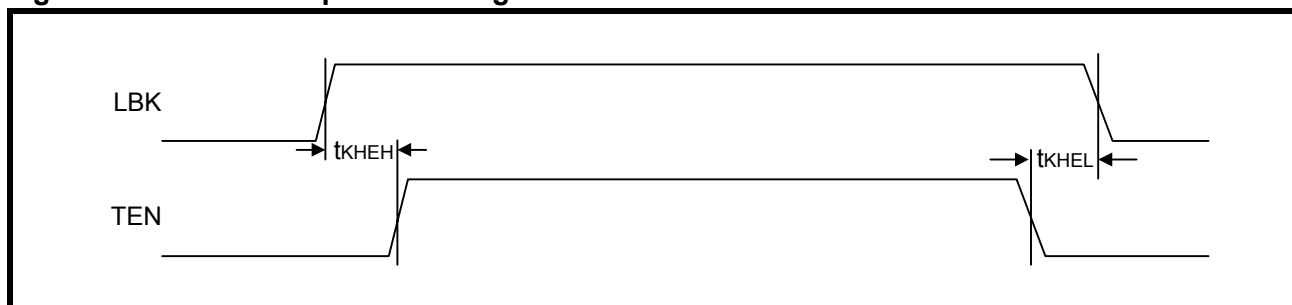
Figure 44: Mode 5 Loopback Timing
