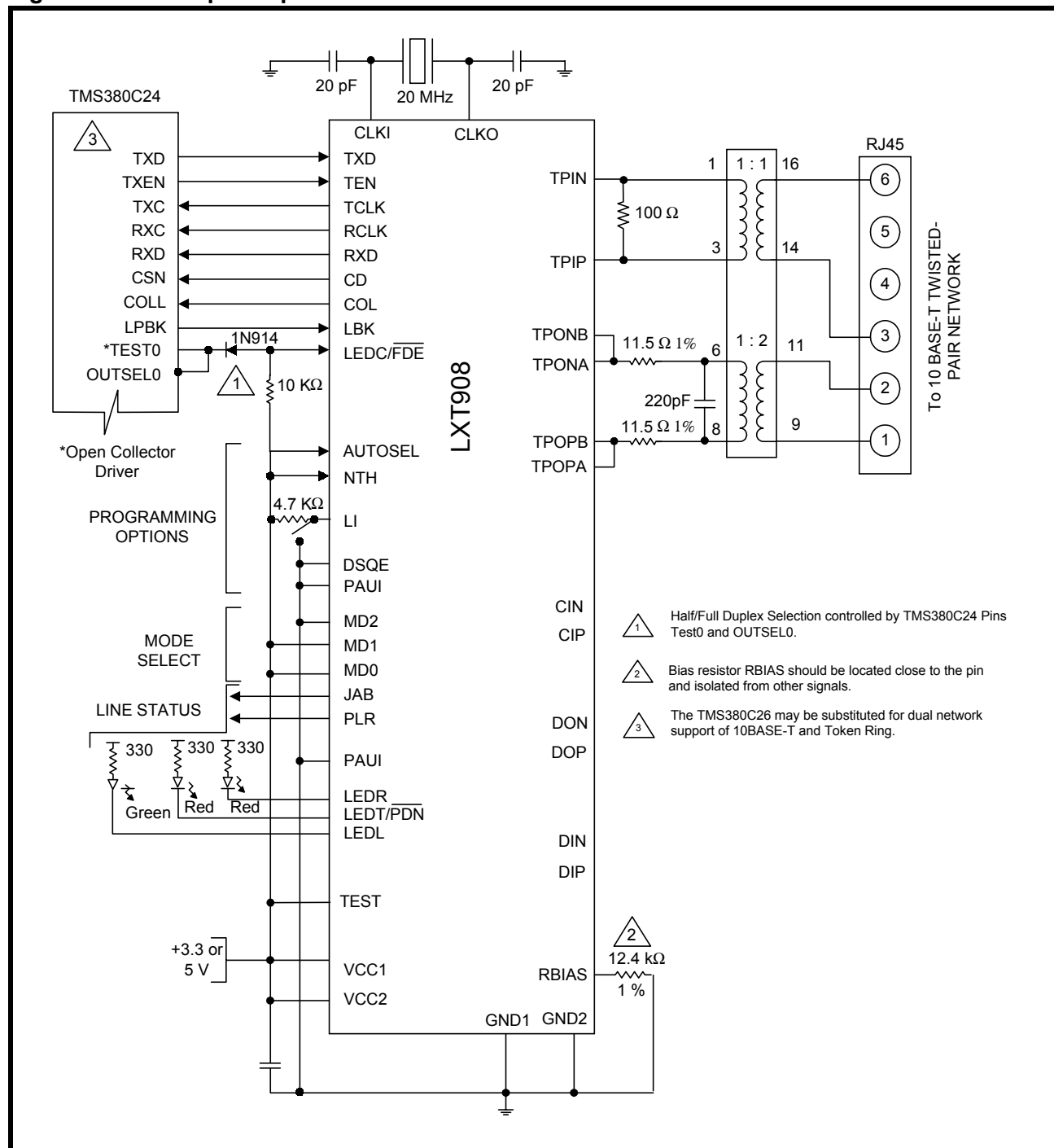
Figure 9: Full-Duplex Operation
