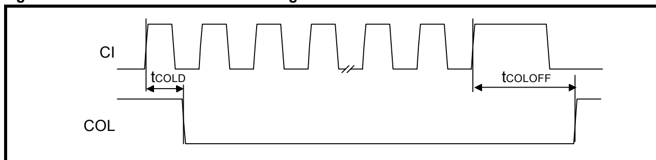
Figure 24: Mode 2 Collision Detect Timing
