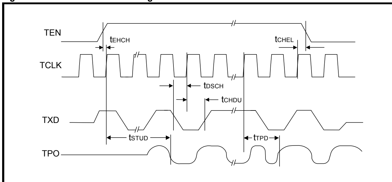
Figure 18: Mode 1 Collision Detect Timing
