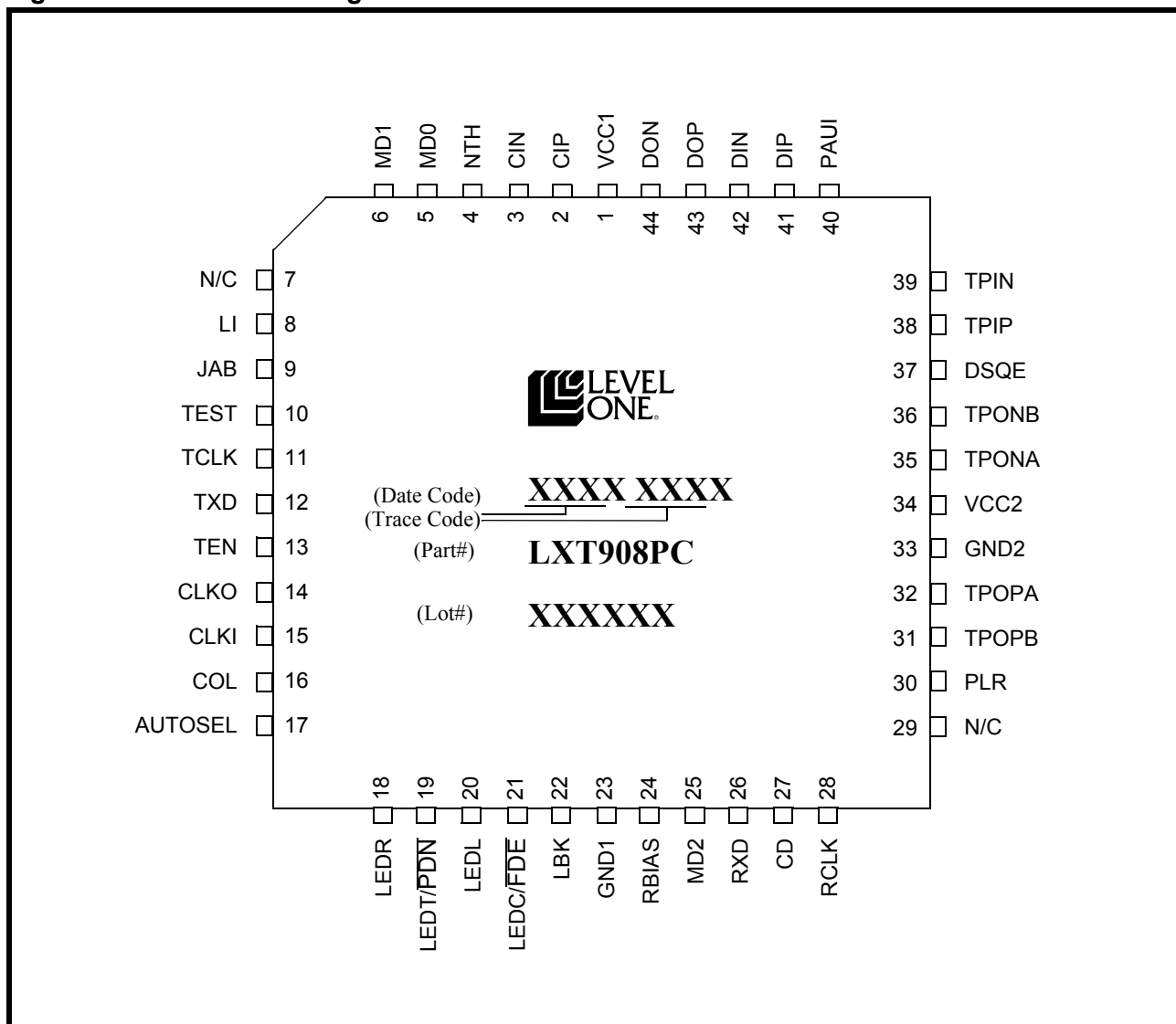
Figure 1: LXT908 Pin Assignments
