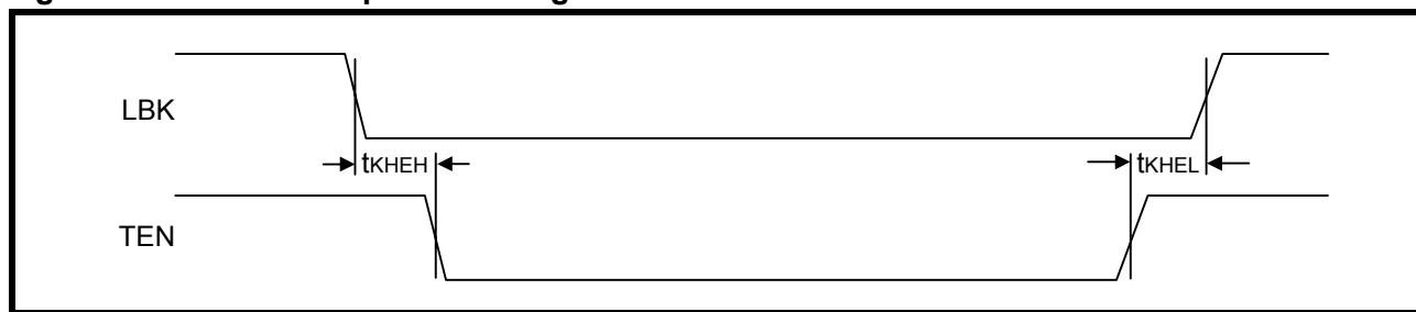
Figure 26: Mode 2 Loopback Timing
