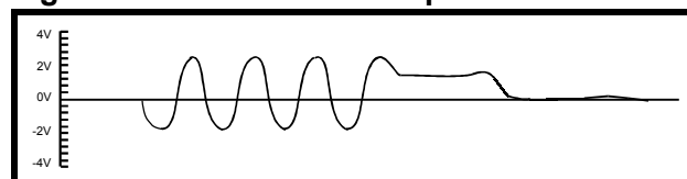
Figure 2: LXT908 TPO Output Waveform
