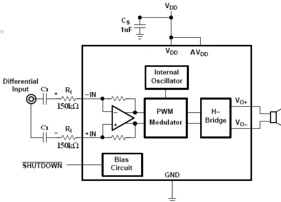
Figure 2. Application Schematic With Differential and Capacitors Input Configuration
