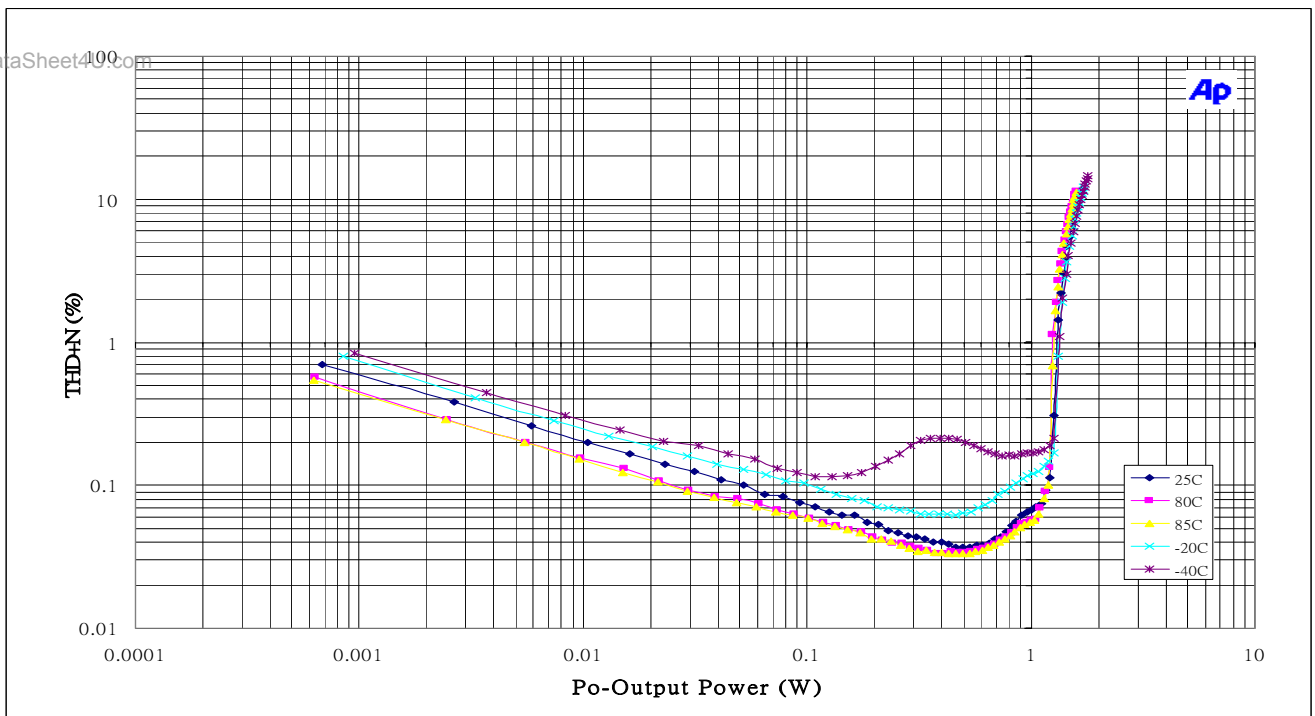
Figure 15 THD+N & Output Power vs Temperature (V DD =5.0V, R L =8Ω)
