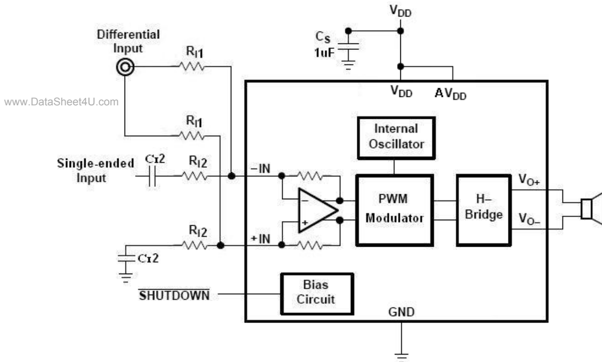
Figure 21. Application Schematic With LY8010 Summing Differential and Sing-Ended Input
