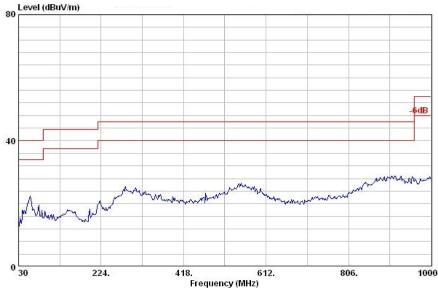
Figure 16 FCC Class-B (Vertical)
