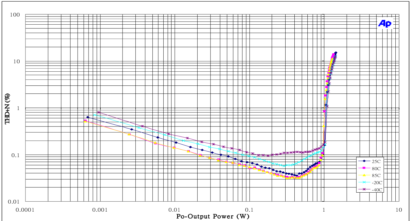
Figure 14 THD+N & Output Power vs Temperature (V DD =4.5V, R L =8Ω)
