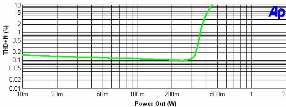
Figure 10 THD+N vs Power Out @ VDD=3V, RL=8Ω, f=1kHz, Av=2
