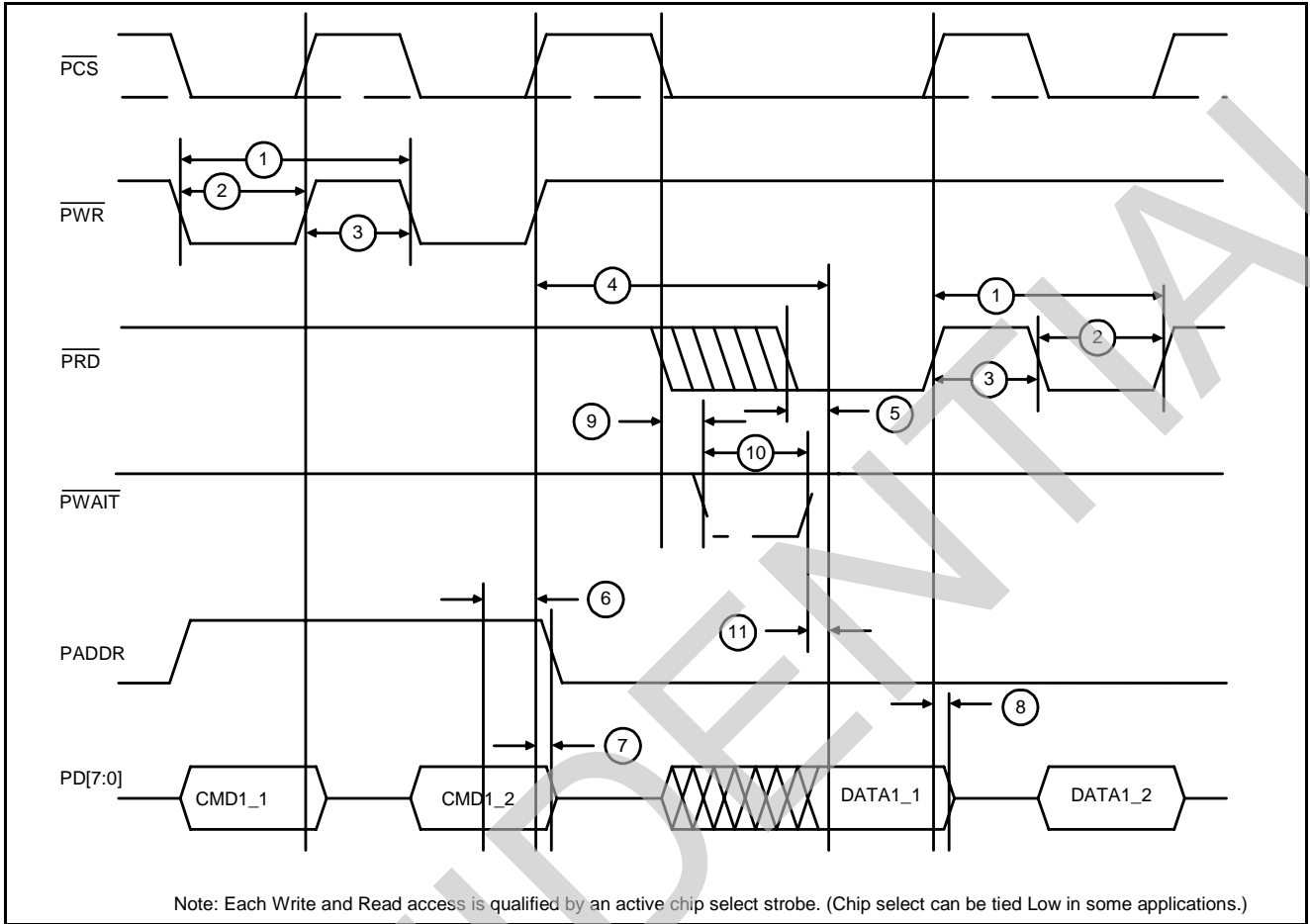
Figure 11 - GPI 8-Bit Read Access Using Separate Read and Write Strokes
