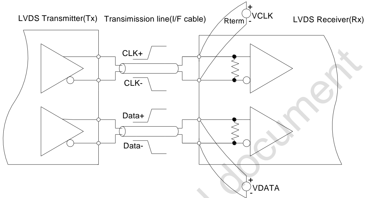
Figure 9 Measurement System
