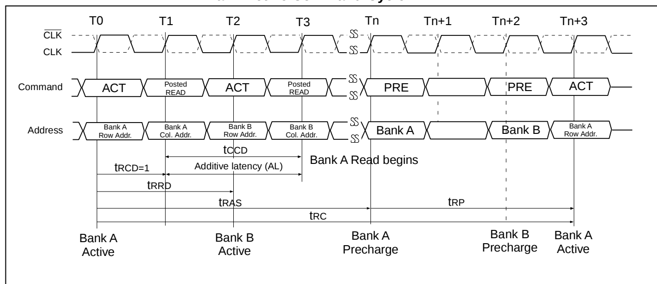
Bank Active Command Cycle
