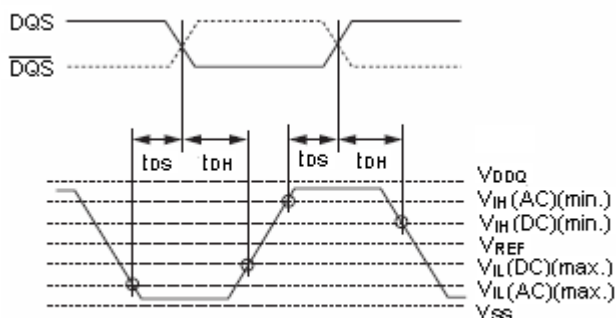
Input Waveform Timing 1 ( t_{\text{DS}} , t_{\text{DH}} )
