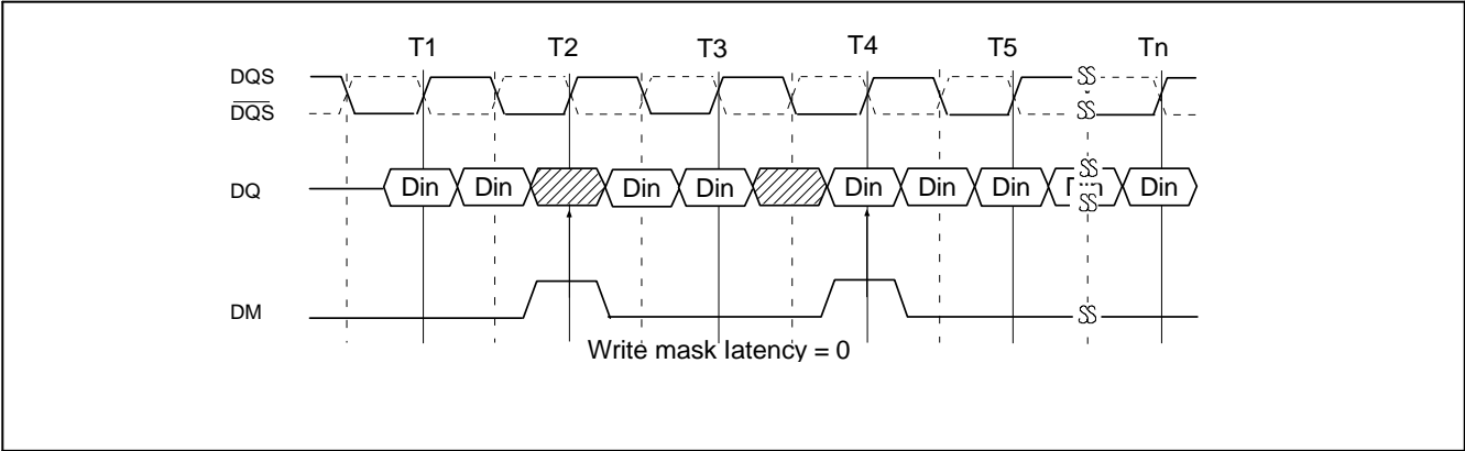
Data Mask Timing
