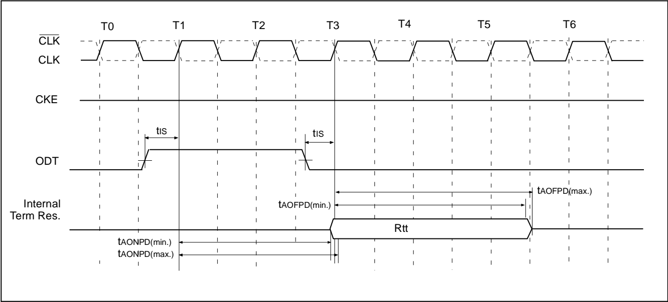
ODT Timing for Power-Down Mode
